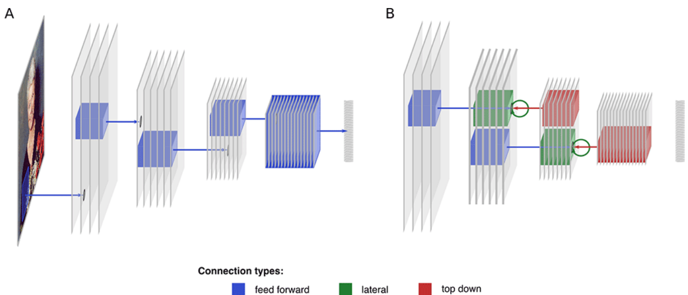
Figure 1. Convolutional neural network structure. (A) An example of a feed-forward convolutional neural network (CNN) with several convolutional layers followed by a fully connected layer. Bottom-up receptive fields for selected neurons are illustrated with blue boxes. (B) The bottom-up (blue), lateral (green), and top-down (red) receptive fields for two example neurons in different layers of a recurrent convolutional neural network (RCNN) are shown.
